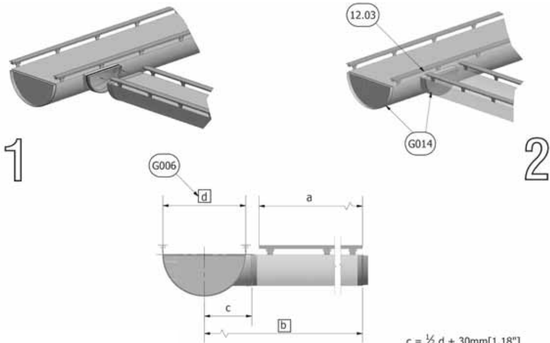
12.13 Type 12 FabricAir® Installation Drawing 2003-1213-000 (2014-FEB)
