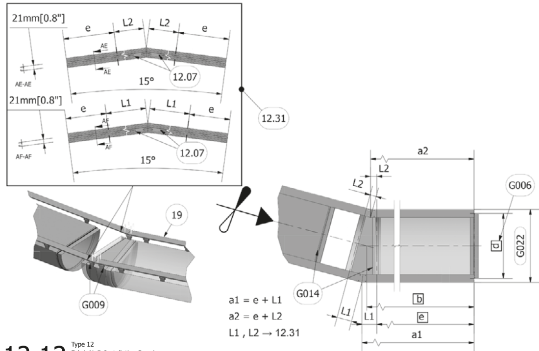
12.12 Type 12 FabricAir® Installation Drawing 2003-1212-000 (2014-FEB)
