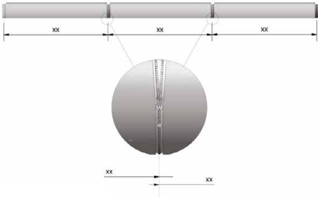
G033 FabricAir® Installation Drawing 2003-G033-000 (2015-JUN)
