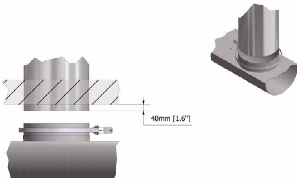
G039 FabricAir® Installation Drawing 2003-G039-000 (2015-JUN)
