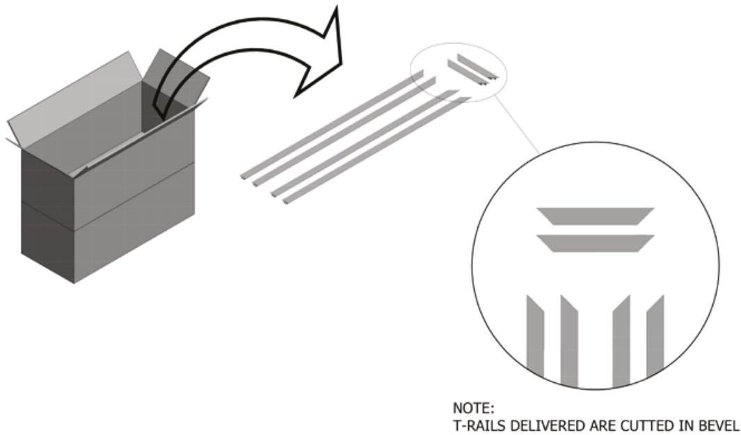
G038 FabricAir® Installation Drawing 2003-G038-000 (2015-JUN)
